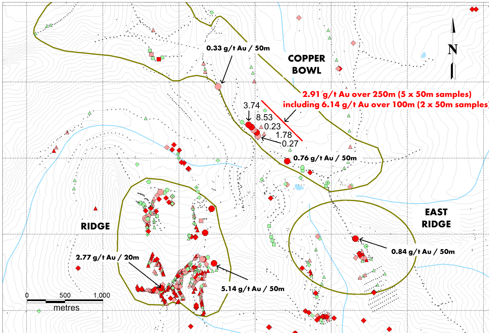
Figure 2 Gold in Rocks and Talus
